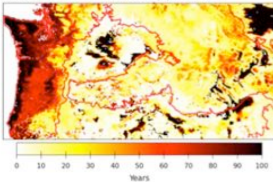
RCP 8.5 With Fire Suppression
