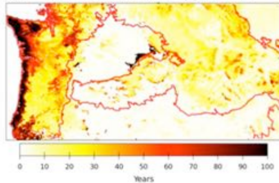
RCP 8.5 Without Fire Suppression
