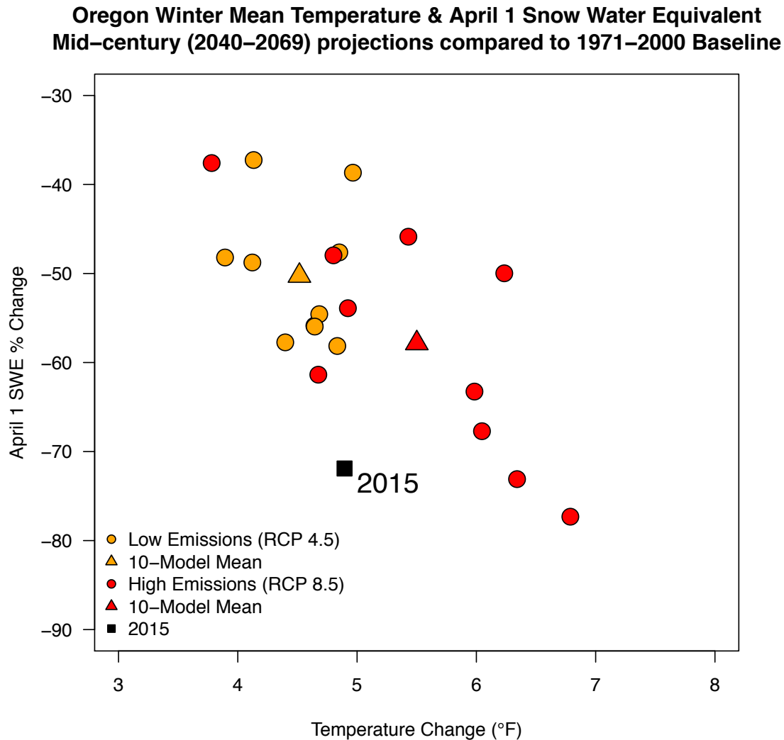
Figure 2.5 Projected future changes in winter (DJF) mean temperature and April 1 snow water equivalent (SWE) averaged over Oregon for mid-century (2040–2069) compared to the 1971–2000 historical baseline. The departure of year 2015 from the 1971–2000 baseline is noted. (Figure source: Meghan Dalton; data source: Mote et al. 2016, updated Livneh et al. , 2015, and http://climate.nkn.uidaho.edu/IntegratedScenarios/ )
