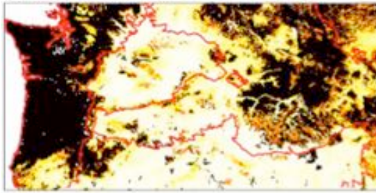
Historical With Fire Suppression
